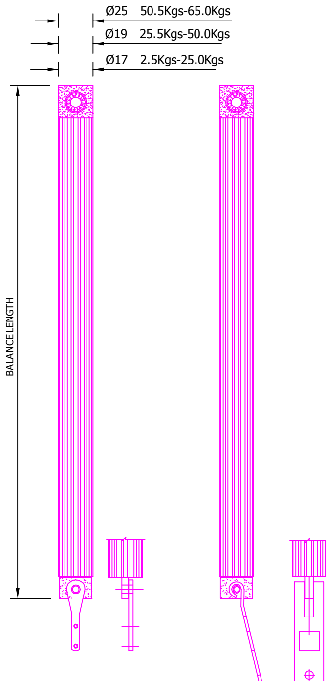
OPTION '1' 2 Pins for tilt in sash. UK105 Torso link bracket.
